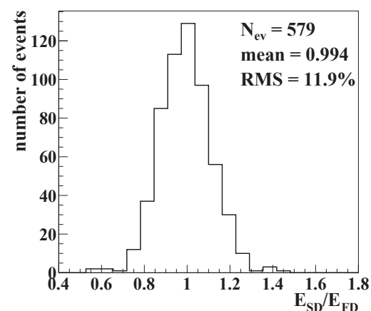
Figure 3. Ratio of the SD to FD energies for the Auger hybrid events above 10^{19} eV [7].
