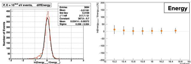
(b) The resolution of Energy ( 3.4 \pm 20.8 \% at 10^{16.0} \text{ eV} ).
