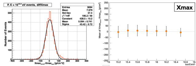
(a) The resolution of X_{\max} ( 5.1 \pm 43.4 \text{ g/cm}^2 at 10^{16.0} \text{ eV} ).
