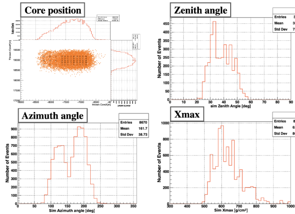
Figure 5: The event distribution of core position (upper left), zenith angle (upper right), azimuth angle (lower left), and X_{\max} (lower right).
