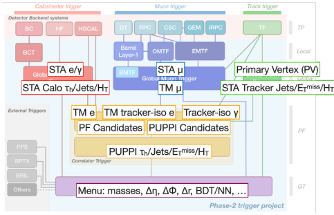
Figure 3: Schematic showing where on the trigger system certain trigger objects are re-constructed. STA is stand-alone, meaning it only take information from one sub-system. TM is track-matched, meaning it takes in information from the tracker and another system. PF and PUPPI combine information from all sub-systems.
