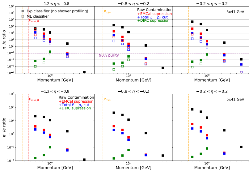
Figure 5. Example of comparative study for different designs of the barrel EM calorimeter using parts of the ePIC software stack. TOP: SciGlass calorimeter technology (courtesy Dmitry Kalinkin). BOTTOM: Imaging calorimeter technology (courtesy Maria Żurek).
