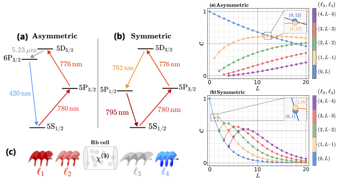
Figure 1. On the left : (a) asymmetric (a) and (b) symmetric Rb 4-level schemes for FWM for pair generation, (c) principle of the experiment. On the right : (a) probability amplitude OAM of the blue (420 nm) in the output pair, and (b) of the NIR (795 nm).
