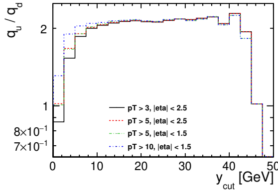
Figure 3. The ratio of the u - and d -type events as a function of y_{cut} for different detector acceptance cuts: (p_T^T > 3 \text{ GeV}, |\eta| < 2.5) – black solid line, (p_T^T > 5 \text{ GeV}, |\eta| < 2.5) – red dashed line, (p_T^T > 5 \text{ GeV}, |\eta| < 1.5) – green dash-double-dotted line, (p_T^T > 10 \text{ GeV}, |\eta| < 1.5) – blue dash-dotted line.
