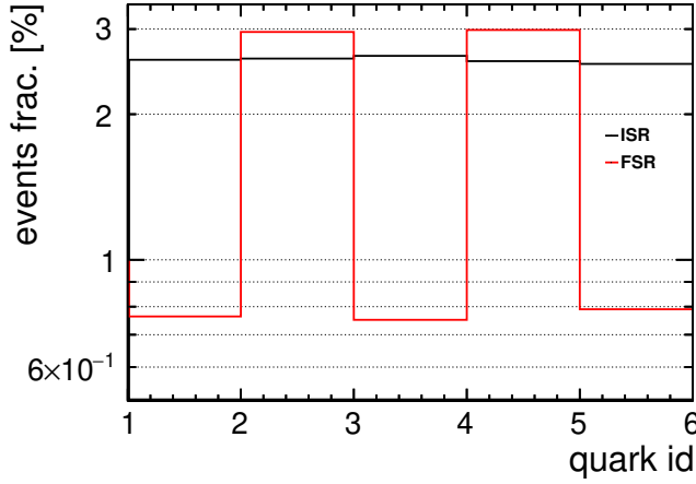
Figure 1. The fraction of events rejected by the matching procedure for different quark flavours (normalised to the cross section per flavour) for ISR (black) and FSR (red)
