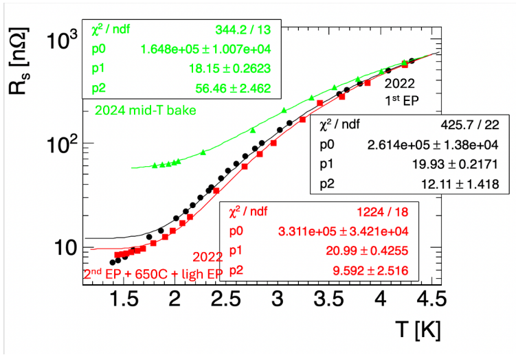
Figure 2. Comparison of surface resistance as a function of temperature before and after mid-T bake. The black circle points show data after 1st EP. The red squares show data after 2nd EP and annealing at 650^\circ\text{C} for 10 hours followed by light EP. The green triangles show the data after mid-T bake newly presented in this article. The solid lines are fitting curves.
