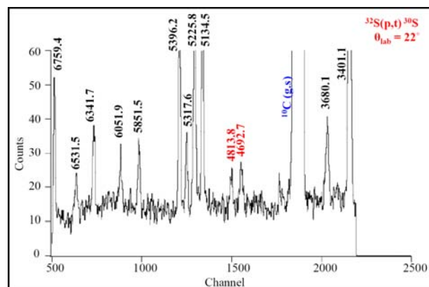
Fig. 1. Focal plane spectra of the ^{32}\text{S}(p,t) reaction corresponding to the states of ^{30}\text{S} , after gating on tritons, shown at selected angle. The background peak of ^{10}\text{C}^{\text{g.s.}} is labeled. The states of ^{30}\text{S} are labeled by their energies averaged over all angles obtained in this work. All energies are in keV. The states of interest are labeled in red.
