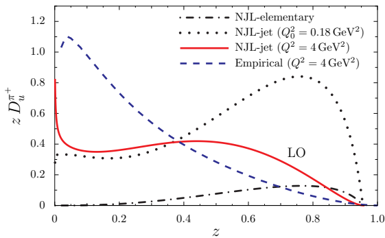
Fig. 5. Favoured fragmentation function zD_u^{\pi^+}(z) . The dash-dotted line is the elementary fragmentation function, and the dotted line is the full fragmentation function in the NJL-jet model. The solid line is the result after LO evolution to Q^2 = 4 \text{ GeV}^2 , and the dashed line is the empirical NLO result of Ref. [5], evolved to Q^2 = 4 \text{ GeV}^2 .
