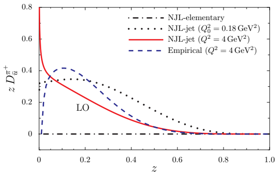
Fig. 6. Unfavoured fragmentation function zD_u^{\pi^-}(z) . The dotted line is the result in the NJL-jet model. The solid line is the result after LO evolution to Q^2 = 4 \text{ GeV}^2 , and the dashed line is the empirical NLO result of Ref. [5], evolved to Q^2 = 4 \text{ GeV}^2 . Note that the elementary fragmentation function vanishes for this case because of charge conservation.
