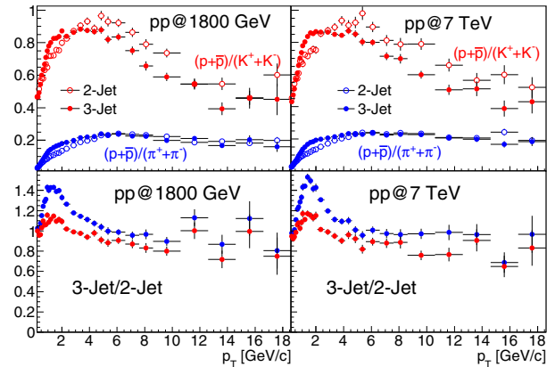
Fig. 3. Top panels: p/\pi (blue) and p/K (red) ratios for all production channels spectrum. Bottom panels: (3\text{-jet ratio})/(2\text{-jet ratio}) .
