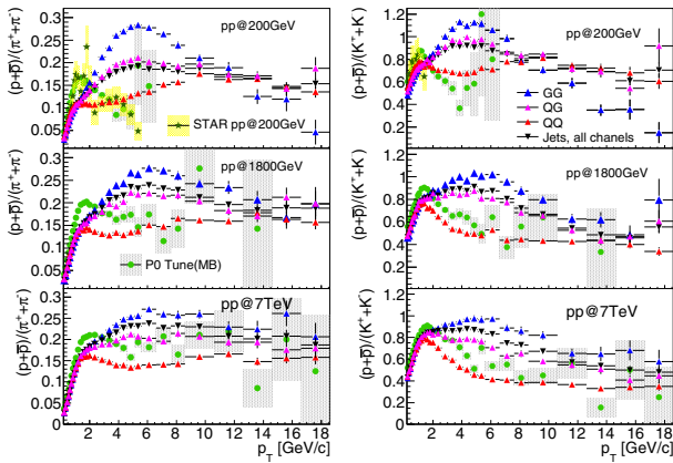
Fig. 1. p/\pi (left panels) and p/K (right panels) for various production channels; GG (blue triangles), QG (magenta triangles), QQ (red triangles) compared to all production channels (black triangles) and MB (green circles). At \sqrt{s} = 200 GeV ratio is compared to STAR data [12]
