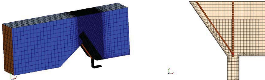
Figure 3: Geometry of mesh for elevation angle 55^\circ (left) and discretization of mesh around nozzle (right). The points define probes for post-processing.
