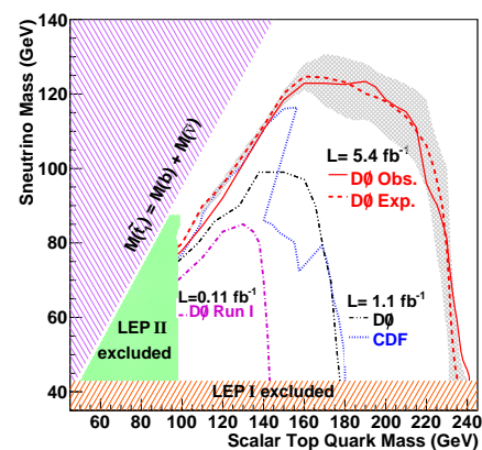
Fig. 1. D0 observed and expected 95% C.L. exclusion contour in the sneutrino and scalar top mass plot, and comparison with previous results.
