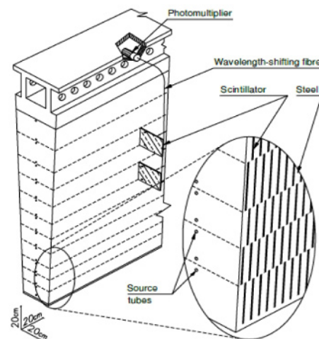
Figure 1. Schematic view of one of the 64 azimuthal modules of TileCal. The module structure and the signal collection system are shown.
