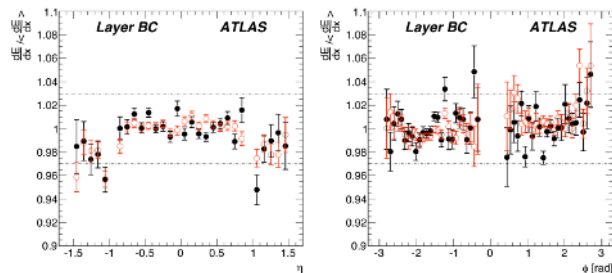
Figure 3. Cell energy uniformity using cosmic muon rays. The TileCal cell energy is uniform within 3% both in \eta and \phi coordinates inside each radial layer. Data (closed circles) are well reproduced by Monte Carlo predictions (open circles). The horizontal lines limit the \pm 3\% bands.
