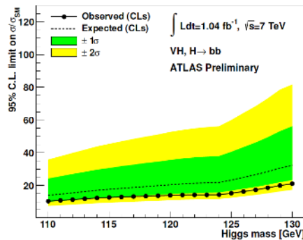
Fig. 2. Expected (dashed) and observed (solid line) exclusion limits for the ZH \rightarrow llb\bar{b} and WH \rightarrow \nu b\bar{b} channels combined, expressed as the ratio to the SM cross section, using the profile-likelihood method with CL_s [3]. The green and yellow areas represent the 1\sigma and 2\sigma ranges of the expectation in the absence of a signal.
