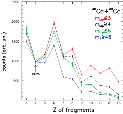
Figure 2: (Color Online) Z distributions of light fragments emitted at \theta_{lab} = 11.5^\circ in ^{40}\text{Ca}+^{40}\text{Ca} events of reaction. Various selections on m_{lcp} have been performed: m_{lcp} \leq 3 (red line), m_{lcp} \geq 4 (black line) and m_{lcp} \geq 6 (green line). HR selection ( m_1 \geq 46 ) is in blue.
