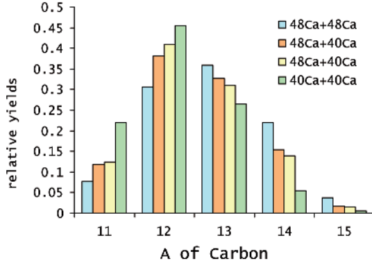
Figure 1: Relative emission yields of Carbon isotopes, emitted at \overline{\theta_{lab}} = 9.3^\circ , in the four studied systems ^{40,48}\text{Ca}+^{40,48}\text{Ca} at 25 MeV/nucleon. Isotopes have been resolved in mass by means of \Delta E - E technique.
