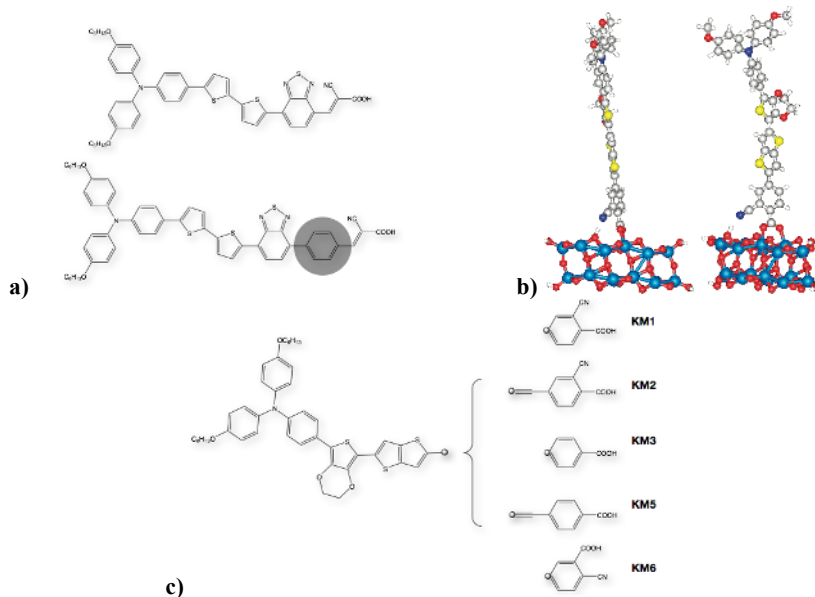
Fig. 1. a) Chemical structures of investigated sensitizers with triphenylamine donors and BTDA/cyanoacrylic acid acceptors. b) Side and front views of the binding modes of a cyanobenzoic acid to \text{TiO}_2 . c) Chemical structures of sensitizers with various benzoic acid derivatives as acceptor/anchoring groups.
