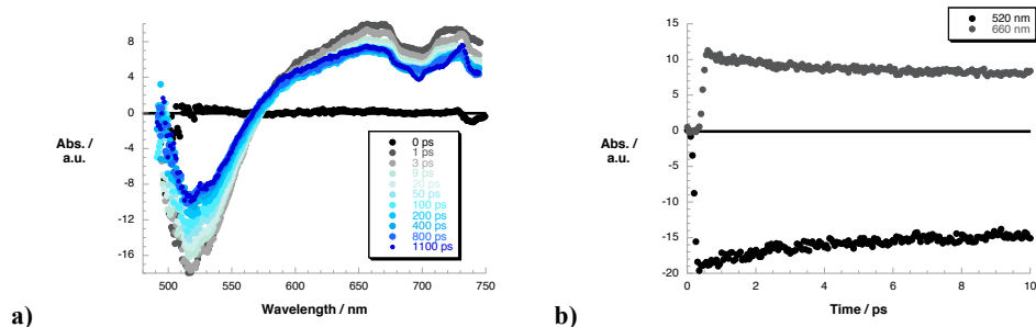
Fig. 1. a) Differential absorption spectrum obtained upon femtosecond flash photolysis ( \lambda_{\text{exc}} = 480 nm) of a film of KM-2 on 3 \mu\text{m} thick TiO 2 with the ground-state transient bleaching between 480 and 560 nm and the TA + cation beyond 580 nm. b) Time-absorption profiles illustrating the charge separation.
