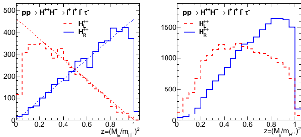
Figure 2. Invariant-mass distributions of \ell\pi_\tau (left) and \ell j_\tau (right) in the pp \rightarrow H^{++}H^{--} \rightarrow \ell^+\ell^+\ell^-\tau^- process followed by hadronic decays of \tau^- , after the requirement of the same-signed dilepton with M_{\ell\ell} \simeq m_{H^{\pm\pm}} . Dashed (Solid) histograms are for H_L^{\pm\pm} ( H_R^{\pm\pm} ). Smooth lines in the left panel are theoretical expectations by using Eqs. (4) with some normalization.
