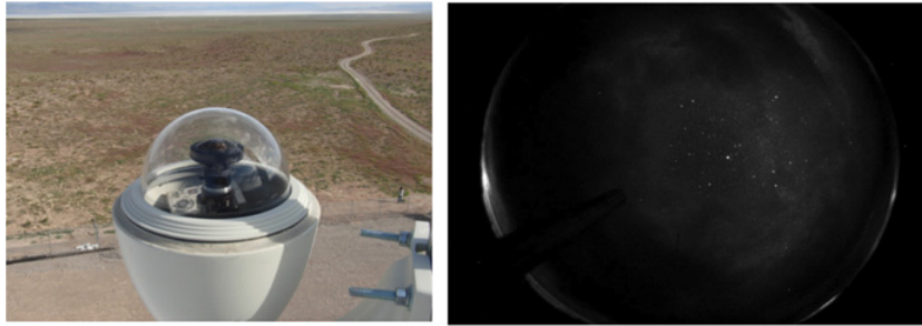
Figure 7. The cloud-ness score by Eye-scan method.
