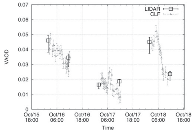
Figure 3. Time variation of VAOD at 8km above the ground.
