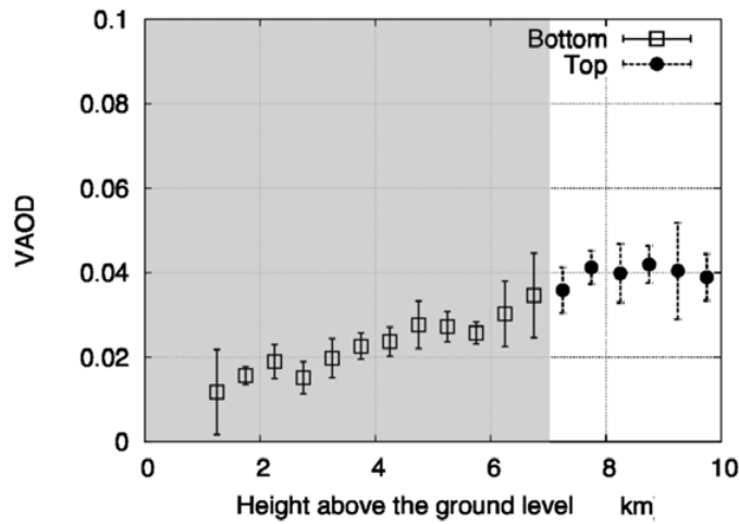
Figure 2. VAOD measured by CLF system as a function of the height.
