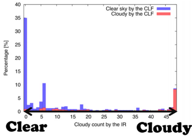
Figure 5. The cloud-ness score by IR camera.
