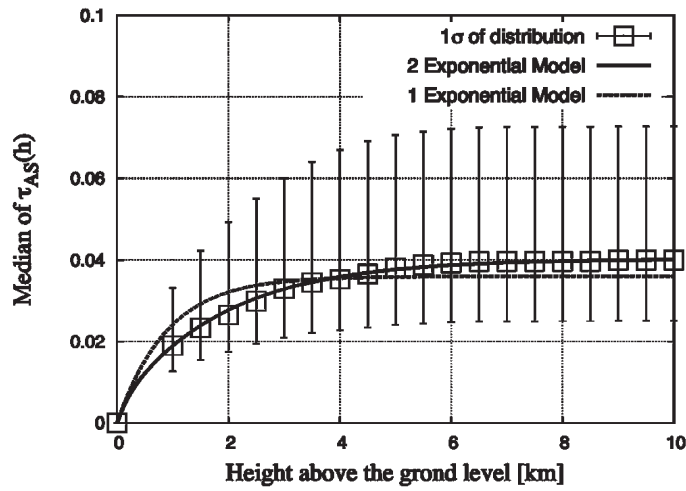
Figure 1. Median of T_{LIDAR}(x) measured by LIDAR system as a function of the height.
