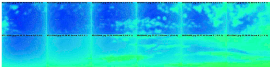
Figure 4. The night sky image by IR camera.
