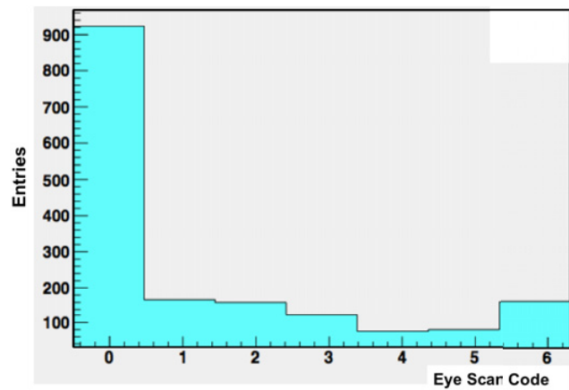
Figure 6. The cloud-ness score by Eye-scan method.
