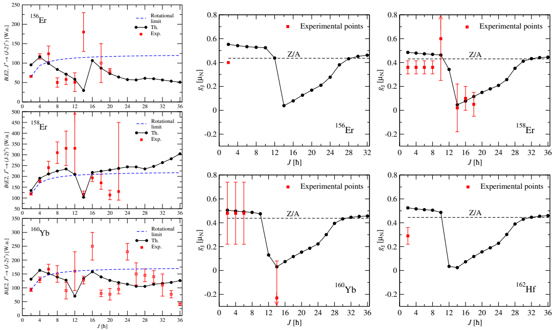
Figure 2. Electromagnetic properties of the treated nuclei along the yrast band. The theoretical results are compared with the available experimental data [9] for E2 probabilities (left) and gyromagnetic factors (right).
