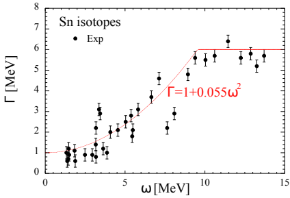
Figure 3. The experimental GT widths of Sn isotopes [8] and their correspondent parameterization.
