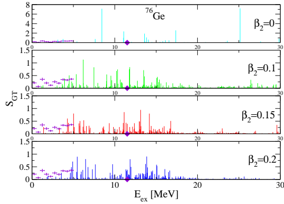
Figure 2. pnQRPA GT strength distributions in ^{76}\text{Ge} obtained with the DIM force for several values of the deformation parameter \beta_2 , including the HFB ground state minimum of \beta_2 = 0.15 . The experimental low energy data [10] as well as the energy position of the main GT peak are also shown.
