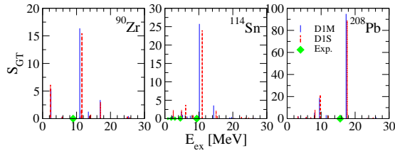
Figure 1. pnQRPA GT strength distributions in ^{90}\text{Zr} , ^{114}\text{Sn} and in ^{208}\text{Pb} calculated the with D1M and D1S forces. The experimental data of the energy peaks position [7–9] are shown as diamonds on the x-axes.
