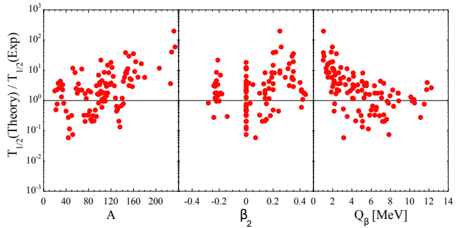
Figure 4. (color online) Ratio between the pnQRPA and experimental \beta^- -decay half-lives as a function of A , \beta_2 and Q_\beta .
