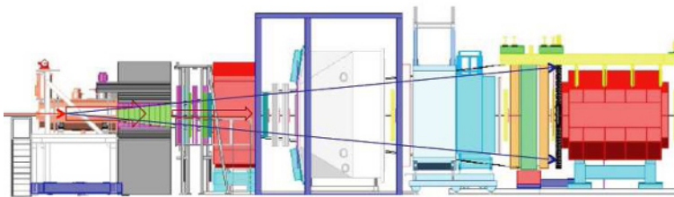
Figure 1. Part of the COMPASS Drell-Yan set-up, including the target. The beam enters from the left-hand side.
