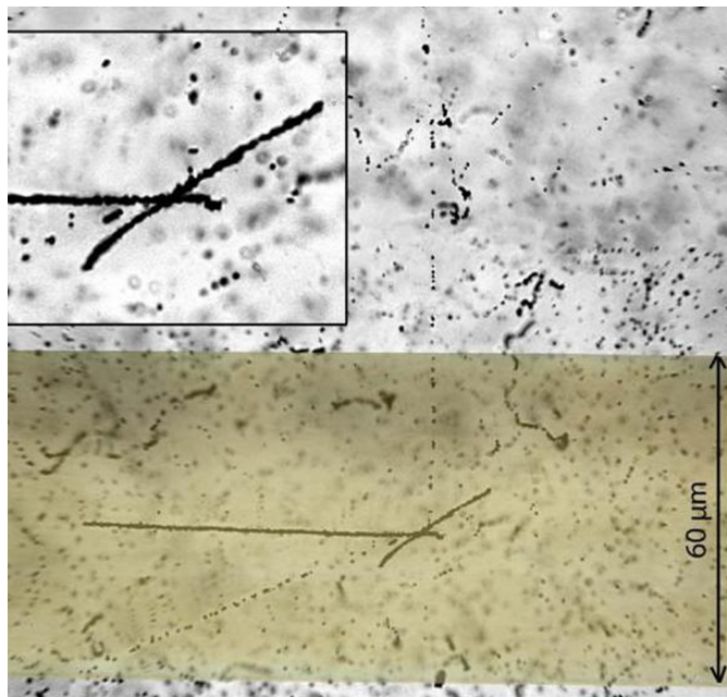
Figure 2. Mosaic macrophotography of a hammer-like decay of {}^8\text{He} nucleus (horizontal track) stopped in nuclear track emulsion. Pair of electrons (point-like tracks) and pair of \alpha -particles (short opposite tracks). On insertion (top): enlarged decay vertex. To illustrate special resolution the image of the decay is superimposed to macrophotography of a human hair of thickness of 60 \mu\text{m} .
