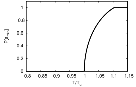
Figure 10. The Polyakov loop P[a^{\min}] calculated at the minimum a = a^{\min} of the effective potential for SU(2) as a function of T/T_c .
