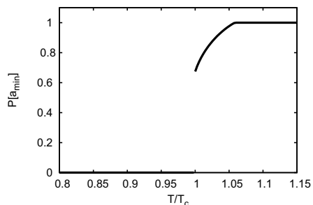
Figure 13. The Polyakov loop P[a^{\min}] calculated at the minimum a = a^{\min} of the effective potential for SU(3) as a function of T/T_c .
