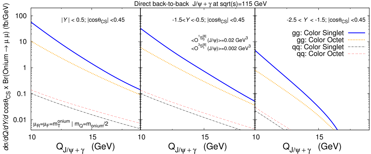
Figure 2: Different contributions to the production of an isolated photon back-to-back with a J/\psi from g-g and q-\bar{q} fusion from the CS and CO channels as a function of the invariant mass of the pair Q_{(J/\psi+\gamma)} for three different rapidity regions (from left to right: |Y| < 0.5 , -1.5 < Y < -0.5 and -2.5 < Y < -1.5 ).
