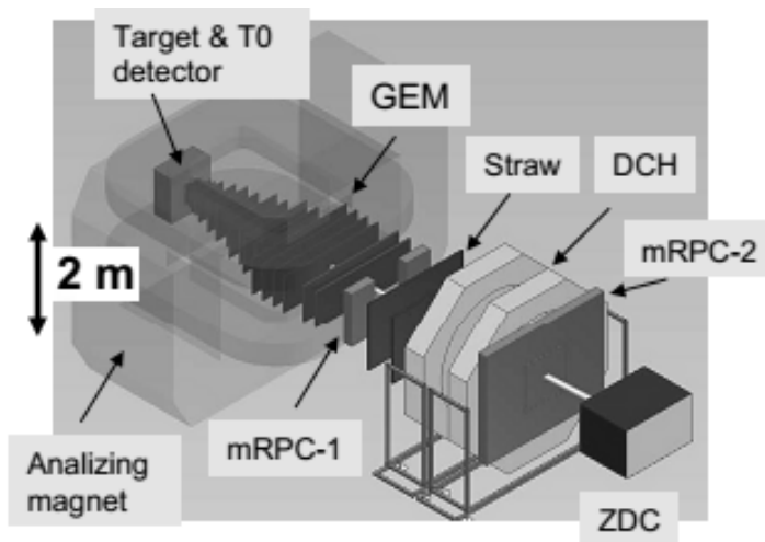
Figure 4. The BM@N setup: GEM – central tracker inside analyzing magnet; DCH+Straw – outer tracker behind the magnet; mRPC+TO – time-of-flight system; ZDC – centrality measurements.
