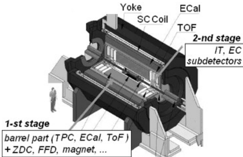
Figure 5. General view of the MPD setup.
