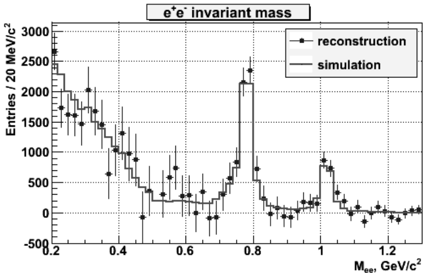
Figure 6. Reconstruction of simulated production of lepton pairs.
