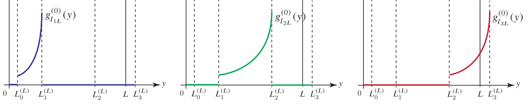
(a) The profiles of triply-degenerated zero modes g_{iL}^{(0)} with M_L > 0 . (The profiles of f_{\nu_{iR}}^{(0)}, f_{e_{iR}}^{(0)} with M_N, M_E < 0 .)
