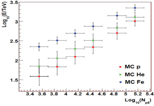
Figure 1. Primary energy as a function of the observed truncated size N_{p8} for simulated showers due to different primary nuclei.
