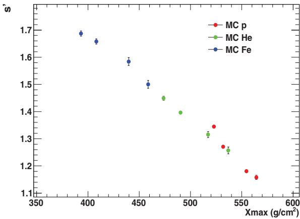
Figure 2. The age parameter s' resulting from the fit of the average LDF for simulated showers vs the corresponding X_{max} average values.
