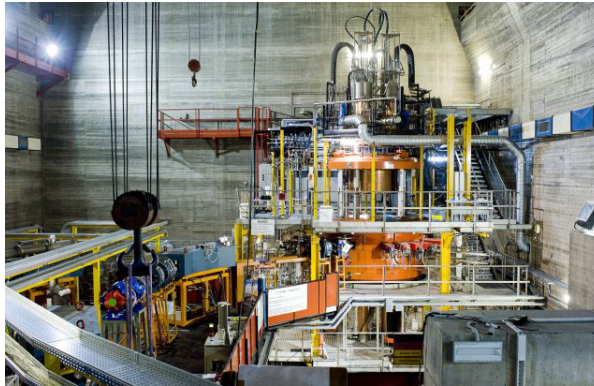
Figure 2: A view of K800 Superconducting Cyclotron at Laboratori Nazionali del Sud in Catania.
