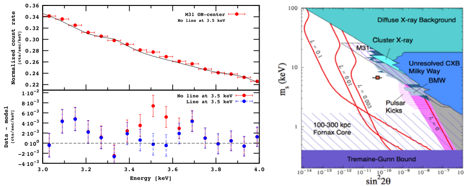
Figure 6. Identification of the 3.5 KeV line in XMM-Newton data (left) and the parameter space of its interpretation in terms of a decaying sterile neutrino. From Ref. [36] and Ref. [35].
