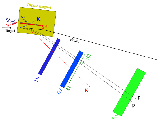
Figure 1. Scheme of the COSY-11 experimental system. Indicated tracks correspond to a simulated ppK^+K^- event.
