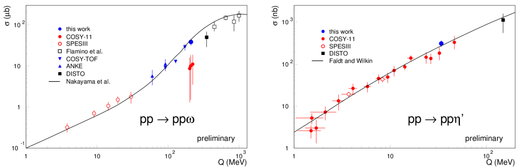
Figure 3. Experimental total cross sections for the \omega production [8–13] and \eta' production [11, 14–19], together with the present data points. Solid lines present theoretical predictions for the \omega and \eta' production cross sections from Ref. [20] and [21], respectively.
