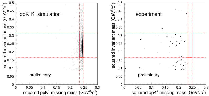
Figure 2. Simulated (left) and measured (right) two-dimensional plots of invariant mass squared of the third (non-proton) particle registered in S1, versus missing mass squared of the ppK^+ system. Red lines present the 3\sigma limits for distribution of the ppK^+K^- events.
