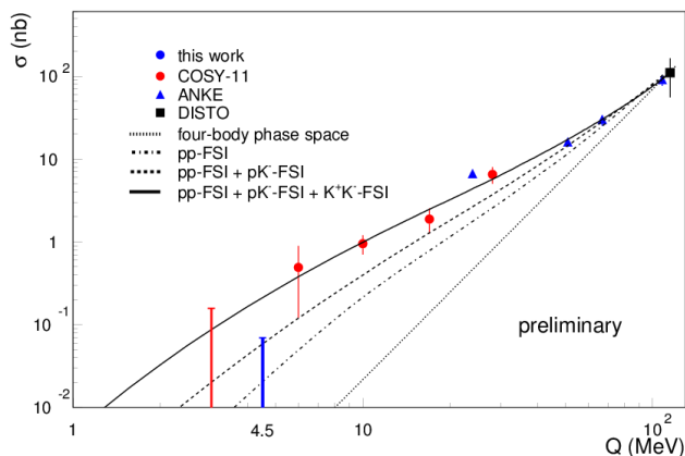
Figure 4. The pp \rightarrow ppK^+K^- excitation function obtained from previous experiments [11, 24–28], together with the present upper limit of the total cross section. The dotted line presents an energy dependence according the phase space volume, the dotted-dashed line incorporates the pp -FSI, the dashed line includes additionally the pK^- -FSI and solid line is obtained by taking into account also the K^+K^- interaction. All theoretical calculations are normalized to the DISTO point at Q = 114 MeV.
