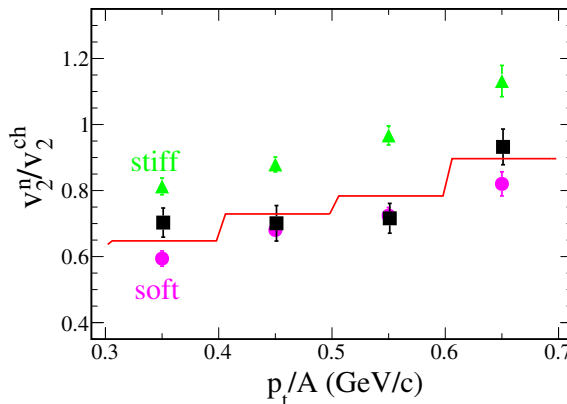
Figure 2. Elliptic flow ratio of neutrons with respect light charged particles for 7.5 fm as a function of the transverse momentum p_t/A . Black squares are experimental data. Triangles and circles are UrQMD predictions respectively for a stiff and soft power-law exponent of the symmetry energy potential.
