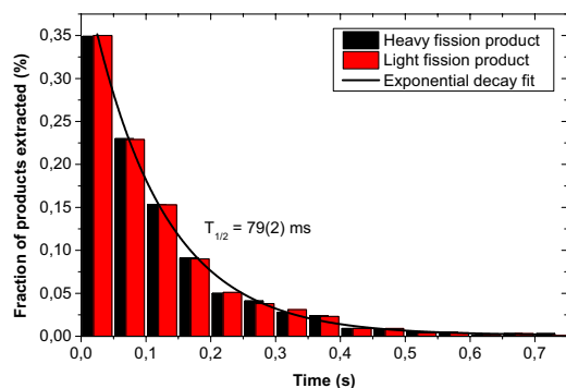
Figure 6. Histogram of evacuation times from the COMSOL ® simulation. The half life of the ions in the ion guide of 79 ms correspond to a mean evacuation time of 113 ms. These numbers seem to be independent of ion mass.
