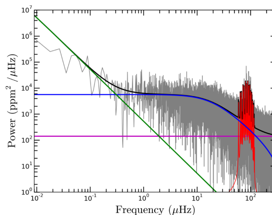
Figure 1: Result of the fit of the power density spectrum (PSD) associated with a Kepler red giant target (KIC 5527304).
