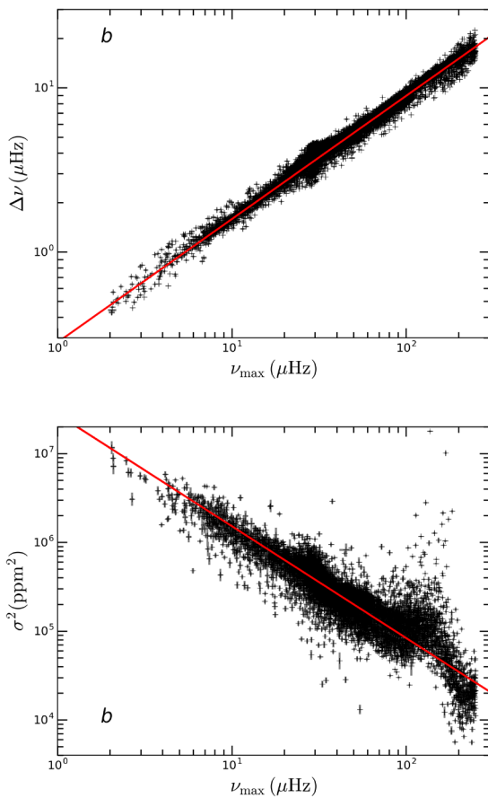
Figure 2: Top: \Delta\nu as a function of \nu_{\max} for about 13,000 Kepler red giants. Bottom: \sigma^2 as a function of \nu_{\max} .
