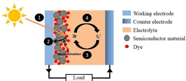
Fig. 1. The structure of DSSC.
