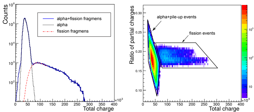
Figure 2. (a) Total integrated charge spectrum, separating \alpha particles and FF; (b) Correlation between the ratio of partial charges and the total integrated charge. PSD improves the discrimination between \alpha particles and FF.
