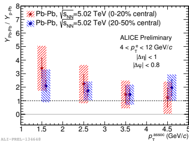
Figure 4: Ratio of near-side associated yields in Pb-Pb (0–20% and 20–50%) and in p-Pb collisions as a function of associated particles p_T .
