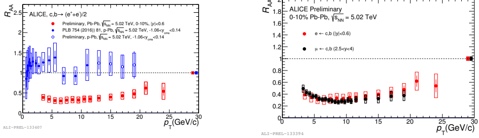
Figure 3: The nuclear modification factor for e^{HF} in Pb-Pb and in p-Pb collisions at \sqrt{s_{NN}} = 5.02 TeV (left), and of e^{HF} ( |y| < 0.6 ) and \mu^{HF} ( 2.5 < y < 4 ) in 0-10% Pb-Pb collisions (right).
