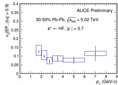
Figure 5: Elliptic flow ( v_2 ) for e^{HF} in semi-central (30-50%) Pb-Pb collisions at \sqrt{s_{NN}} = 5.02 TeV.
