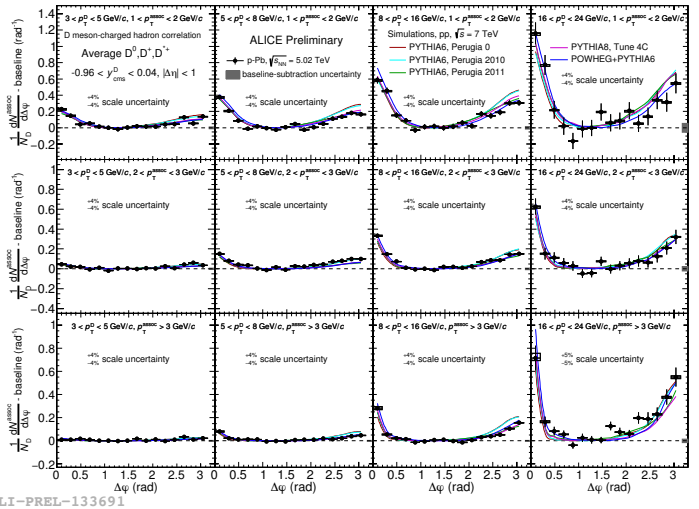
Figure 2: The azimuthal correlation of D mesons with charged particles in p–Pb collisions at \sqrt{s_{NN}} = 5.02 TeV.
