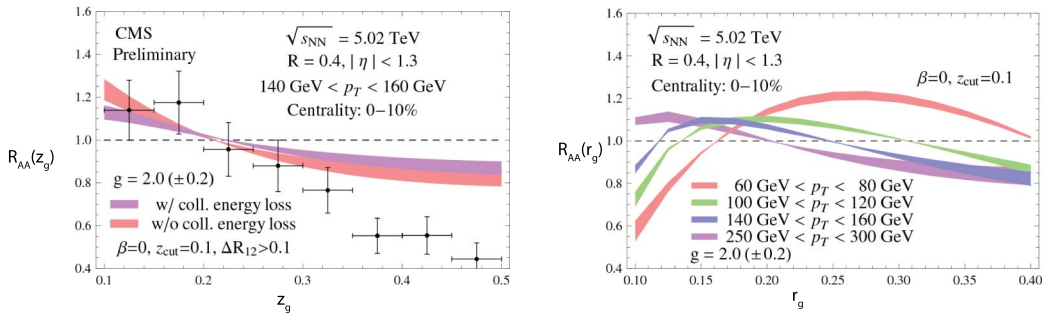
Figure 4. Left panel: theoretical calculations compared to preliminary CMS data for the ratio of momentum sharing distributions of inclusive anti- k_T R = 0.4 jets in central Pb+Pb and p+p collisions at \sqrt{s_{NN}} = 5.02 TeV. Purple and red bands correspond to calculations with and without the implementation of collisional energy loss. Right panel: the groomed jet radius modification of inclusive jets in proton-proton and central lead-lead collisions at \sqrt{s_{NN}} = 5.02 TeV. We show results for four p_T bins with 60 \text{ GeV} < p_T < 80 \text{ GeV} , 100 \text{ GeV} < p_T < 120 \text{ GeV} , 140 \text{ GeV} < p_T < 160 \text{ GeV} and 250 \text{ GeV} < p_T < 300 \text{ GeV} .
