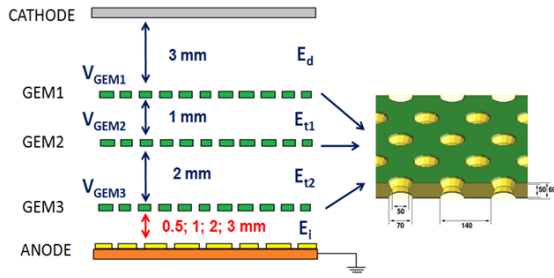
Figure 1. Triple GEM beam monitor set up.
