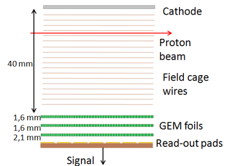
Figure 9. 13 TPG prototype schema. The beam cross the detector through two mylar windows.
