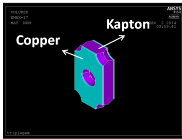
Figure 2. Unit cell of GEM foil simulated with ANSYS showing copper part (light blue) and kapton part (violet).
