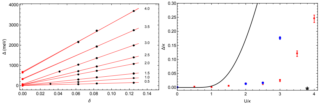
Figure 4. (Left) The dependence of the gap \Delta on \delta = \beta/N_t from the (15,15) tube (black points, error bars too small to be seen), and their continuum extrapolation (red points). The different lines represent calculations with different Hubbard ratios, with the lowest being U/\kappa = 0.5 and highest U/\kappa = 4 , as labelled in the figure. (Right) The dependence of the Mott-insulating gap \Delta (in units of \kappa ) on Hubbard ratio U/\kappa for (15,15) tube (red squares) and (10,10) tube (blue circles). The solid line shows the limiting 1-D analytical result obtained using the Bethe ansatz. Also indicated in the right plot is the location of the critical coupling (black star) for the 2-D hexagonal Hubbard model [12]. The red points of the two plots coincide with each other. [13, 14].
