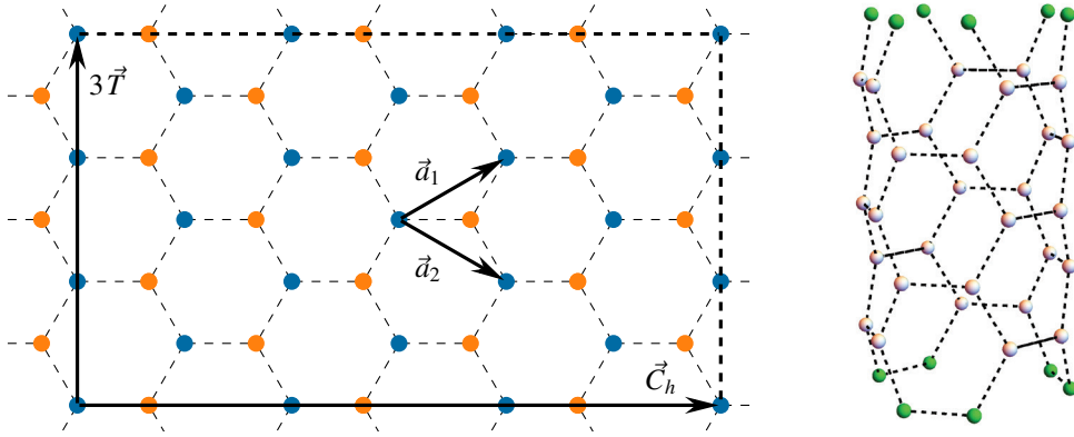
Figure 1. (Left) The basis vectors \vec{a}_1 and \vec{a}_2 and an example \vec{T} and \vec{C}_h vectors used to cut the hexagonal sheet for the (3,3) geometry. (Right) The corresponding tube after subsequent rolling of sheet, and periodic boundary conditions are applied at the green lattice sites.
