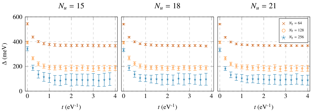
Figure 3. Value of the gap determined from the effective mass at the Dirac point with coupling U/\kappa = 1 and \beta = 8 \text{ eV}^{-1} for N_u = 15, 18, 21 and N_t = 64, 128, 256 . Results are nearly independent in N_u for this (weak) value of the coupling, but demonstrate strong dependence on N_t .
