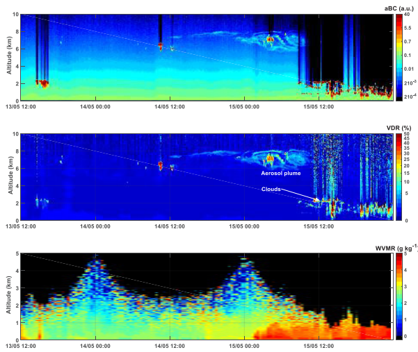
Figure 4. Temporal evolutions, between 13th and 16th May 2016 of the lidar-derived aBC, VDR and WVMR (top, middle and bottom panels, respectively).
