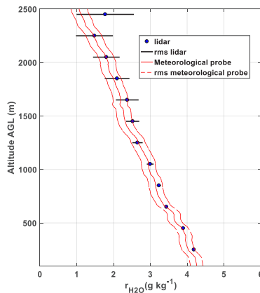
Figure 5. WVMR vertical profiles derived from WALI and the VAISALA™ probe on 5th May 2016. The red dotted line and the horizontal bars delimit the standard deviation on the meteorological probe and the lidar measurements, respectively.
