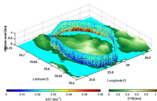
Figure 3. AEC retrieved from the flight around Hammerfest on 16th May 2016.
