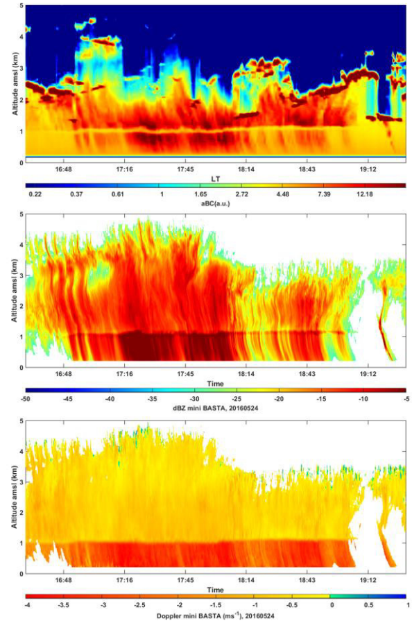
Figure 6. Temporal evolutions on 24th May 2016 of the lidar-derived aBC (top panel), radar reflectivity in dBZ (middle panel), and Doppler radar-derived vertical drop speed (bottom panel).
