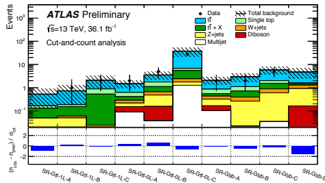
Figure 12: Comparison of the observed data and predicted background event yields in the SRs in the multi- b analysis [17]. Each bin indicates yields in one SR. The bottom panel shows the difference between observed data yields and the total predicted background yields divided by total uncertainties.
