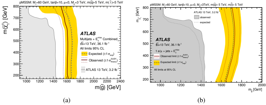
Figure 10: Exclusion limits for gluino pair-production in a scenario of pMSSM model obtained from (a) the 0-lepton (7-11 jets) analysis [13] and from (b) 9-jets signal regions of the 1-lepton analysis [16]. In this pMSSM scenario, M_1 = 60 GeV, \tan\beta = 10 , \mu < 0 , M_2 = 3 TeV, the squark mass= 5 TeV and the slepton mass= 5 TeV are assumed. X-axis and y-axis indicate masses of gluino and chargino appearing in the decay chain. Results are compared with the observed limits obtained by the previous ATLAS searches with the 0-lepton analysis [24] and the 1-lepton analysis [23].
