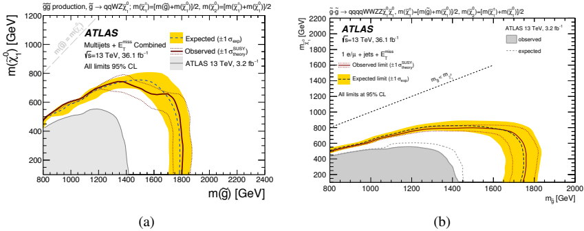
Figure 11: Exclusion limits for gluino pair-production with two-step cascade decay obtained from (a) the 0-lepton (7-11 jets) analysis [13] and from (b) 9-jets signal regions of the 1-lepton analysis [16]. and the result is compared with the observed limits obtained by the previous ATLAS searches with the 1-lepton analysis [23].
