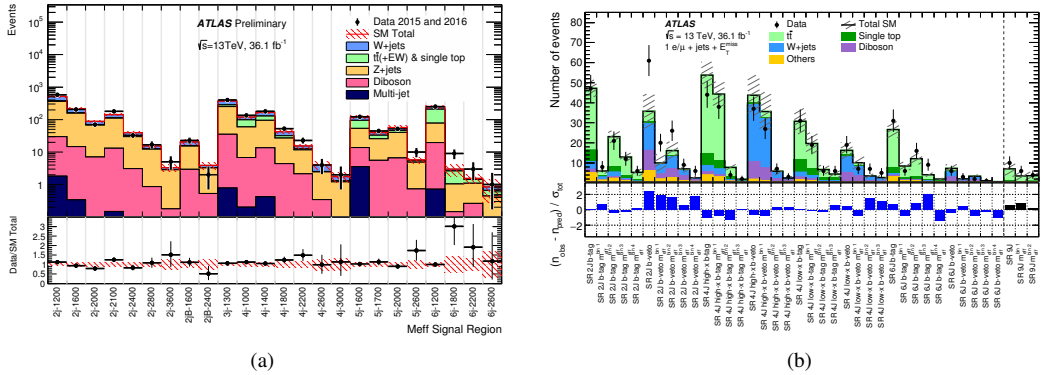
Figure 4: Comparison of the observed data and predicted background event yields in (a) signal regions of the 0-lepton (2–6jets) analysis [9], and (b) signal regions of the 1-lepton analysis [16]. Each bin indicates a yield in one signal region. The bottom panel in Figure (a) shows the ratio of observed data yields to the total predicted background yields, and that in Figure (b) shows the difference between the observed data yields and the predicted total background yields divided by total uncertainties. The regions in Figure (b) are all of the signal regions in the 1-lepton analysis including at least 9jets regions described in Section 3.
