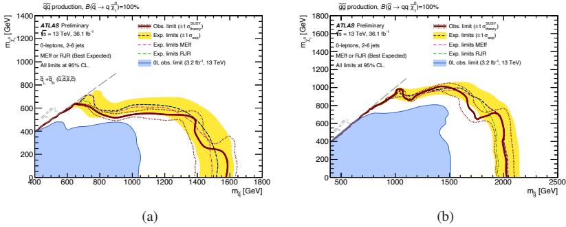
Figure 5: Exclusion limits for (a) light-flavor squark pair-production with direct decay and (b) gluino pair-production with direct decay from the 0-lepton (2–6 jets) analysis [9]. Expected limits from Meff and R-jigsaw-based searches separately are shown. Results are compared with the observed limits obtained by the previous ATLAS searches with the 0-lepton (2–6 jets) analysis [21].
