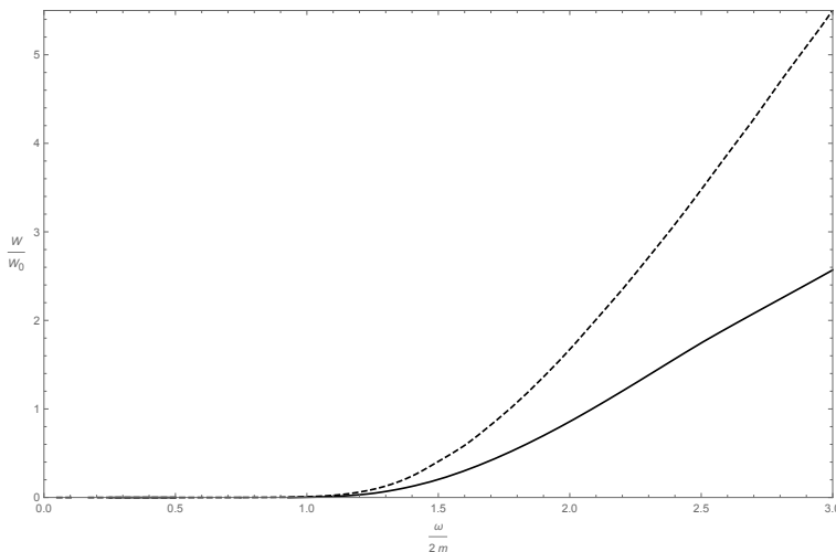
Figure 2. The photon absorption rate due to the channel \gamma_1 \rightarrow \gamma_1\gamma_2 in a strong magnetic field ( B/B_e = 200 ). Dashed line corresponds to the probability in magnetized vacuum without positronium influence [7]. Here W_0 = (\alpha/\pi)^3 m \approx 3.25 \cdot 10^2 \text{cm}^{-1} .
