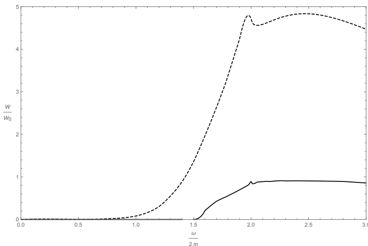
Figure 3. The photon absorption rate due to the channel \gamma_1 \rightarrow \gamma_2\gamma_2 in a strong magnetic field ( B/B_e = 200 ). Dashed line corresponds to the probability in magnetized vacuum without positronium influence [7]. Here W_0 = (\alpha/\pi)^3 m \approx 3.25 \cdot 10^2 \text{cm}^{-1} .
