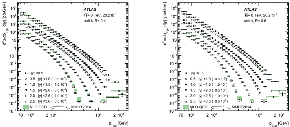
Figure 3. Inclusive jet cross-section as a function of jet p_T in bins of jet |y| in pp collisions at \sqrt{s} = 8 TeV. The results are shown for jets identified using the anti- k_t algorithm with (left) R = 0.4 and (right) R = 0.6 . For better visibility the cross-sections are multiplied by the factors indicated in the legend. The data are compared to the NLO QCD prediction with the MMHT2014 PDF set. The error bars indicate the statistical and the systematic uncertainties in the measurement added in quadrature. The statistical uncertainty is shown separately by the inner vertical line. Taken from Ref. [4].
