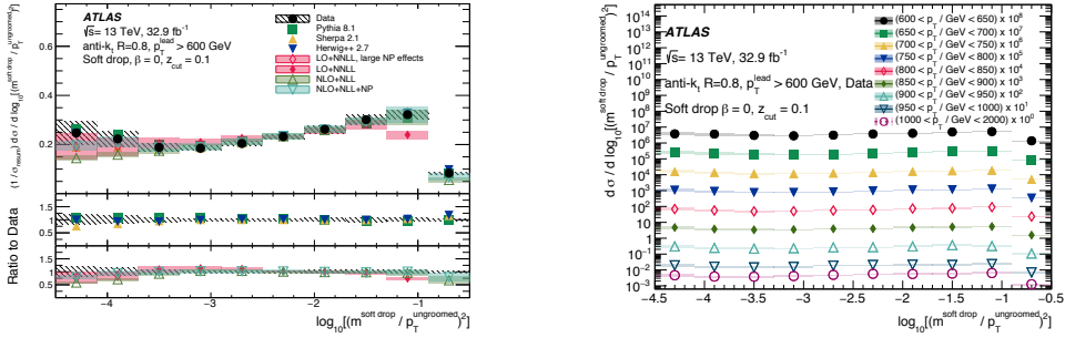
Figure 8. (Left) The unfolded \log_{10}(\rho^2) distribution for anti- k_t R = 0.8 jets with p_T^{\text{lead}} > 600 GeV, after the soft drop algorithm is applied for \beta = 0 , in data compared to PYTHIA, SHERPA, and HERWIG++ particle-level, and NLO+NLL+NP and LO+NNLL theory predictions. The LO+NNLL calculation does not have NP corrections; the region where these are expected to be large is shown in an open marker, while regions where they are expected to be small are shown with a filled marker. The distributions are normalized to the integrated cross section, \sigma_{\text{resum}} , measured in the resummation region, -3.7 < \log_{10}(\rho^2) < -1.7 . The NLO+NLL+NP cross-section in this resummation regime is 0.14 nb for \beta = 0 . (Right) The unfolded \log_{10}(\rho^2) distribution in data for each of the p_T bins in the analysis, overlaid with a multiplicative factor indicated in the legend. Taken from Ref. [7].
