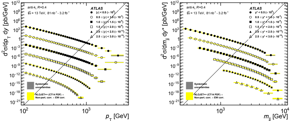
Figure 1. Inclusive (left) jet and (right) dijet cross-sections as a function of p_T for jet and m_{jj} for dijet and |y| , for anti- k_i jets with R = 0.4 in pp collisions at \sqrt{s} = 13 TeV. The statistical uncertainties are smaller than the size of the symbols used to plot the cross-section values. The dark gray shaded areas indicate the experimental systematic uncertainties. The data are compared to NLO pQCD predictions calculated using NLOJET++ with p_T^{\max} for jet and p_T^{\max} \exp(0.3 y^*) for dijet as the QCD scale and the CT14 NLO PDF set. The yellow shaded areas indicate the predictions with their uncertainties. At low and intermediate p_T bins the experimental systematic uncertainties are comparable to the theory uncertainties (drawn on top) and therefore are barely visible. In most m_{jj} bins the experimental systematic uncertainty is smaller than the theory uncertainties and is therefore not visible. Taken from Ref. [3].
