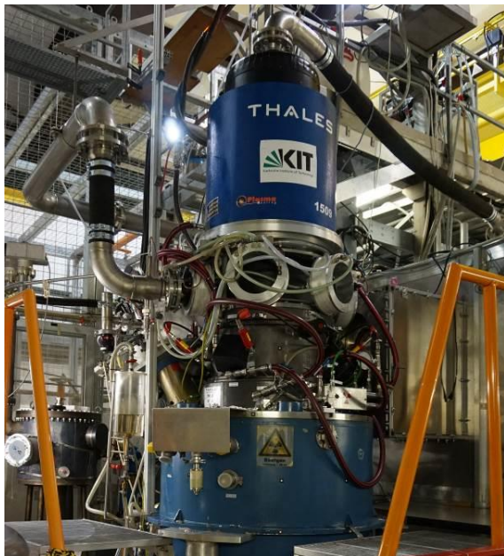
Fig. 6. The EU 1MW, 170 GHz CW industrial prototype gyrotron installed at the KIT superconducting magnet.
