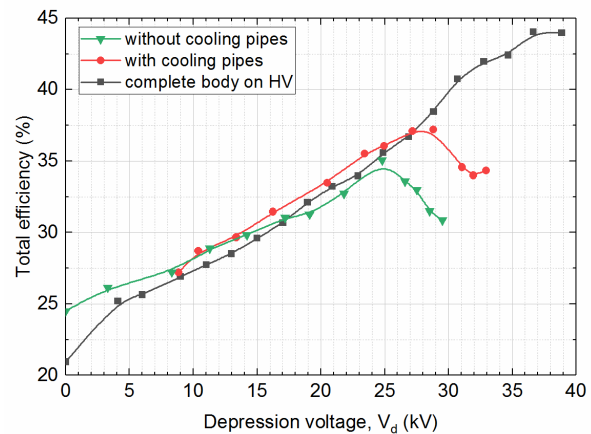
Fig. 5. Measured total efficiency (in depressed collector operation) with respect to the depression voltage for difference configurations of the SP prototype gyrotron (LVOP with average output power approximately 850 kW).
