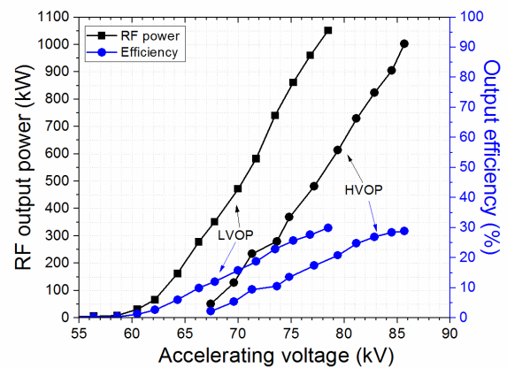
Fig. 2. RF power and corresponding efficiency (in non-depressed collector operation) with respect to the accelerating voltage for the LVOP ( V_{acc} \approx 78 kV, I_b \approx 45 A) and the HVOP ( V_{acc} \approx 86 kV, I_b \approx 40 A).
