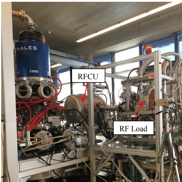
Fig. 9. The EU 1MW, 170 GHz CW industrial prototype gyrotron installed at the SPC superconducting magnet. The gyrotron is connected to the RF load using an RFCU under vacuum.
