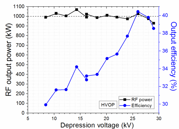
Fig. 3. RF power and corresponding total output efficiency (in depressed collector operation) with respect to the depression voltage for the HVOP ( V_{acc} \approx 86 kV and beam current I_b \approx 43 A).
