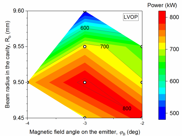
Fig. 7. RF power with respect to the magnetic field angle at the emitter and the radius of the electron beam in the cavity. Operation at the LVOP with long pulses (> 60 s).
