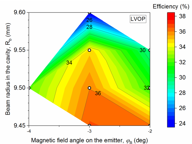
Fig. 8. Total efficiency with respect to the magnetic field angle at the emitter and the radius of the electron beam in the cavity. Operation at the LVOP.
