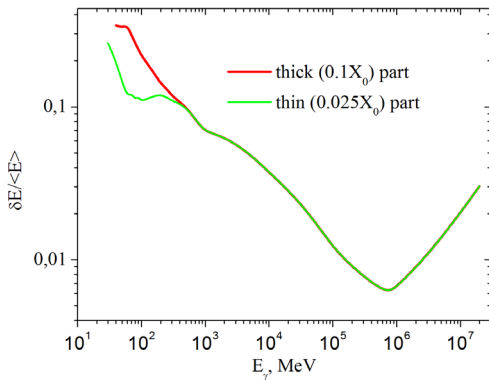
Figure 5. The dependence of the energy resolution vs the energy for two parts of the converter: 4 panels with W=0.025X_0 and 7 panels with W=0.1X_0
