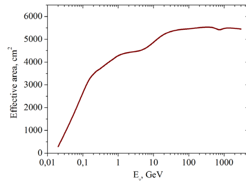
Figure 3. The dependence of the effective area vs the energy for vertically incident particles
