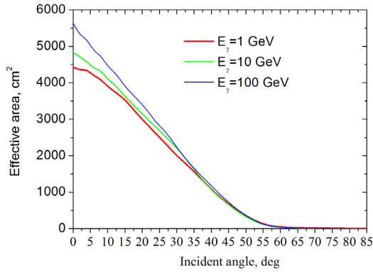
Figure 4. The dependence of the effective area vs the angle of incidence of particles for E_\gamma = 1 GeV; E_\gamma = 10 GeV; E_\gamma = 100 GeV
