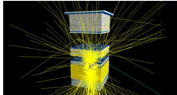
Figure 2. The interaction of the 100-GeV gamma ray with the GAMMA-400 matter with the formation of backscattering particles. Secondary gammas, positrons and electrons are marked by yellow, violet and blue colors respectively
