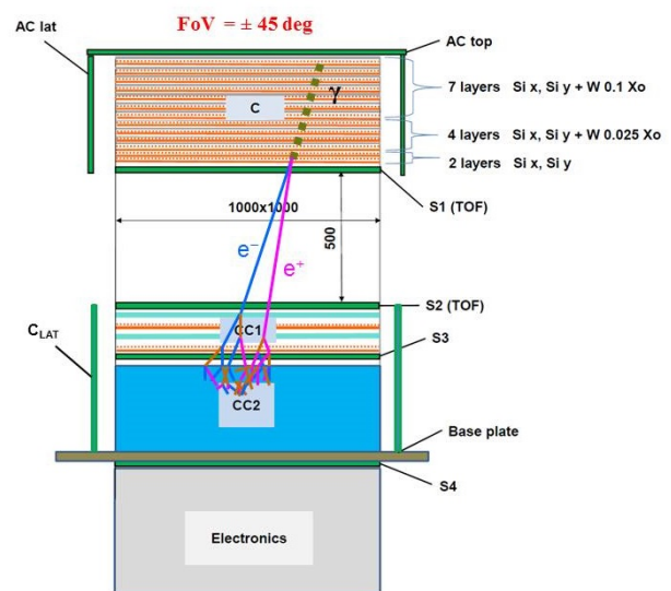
Figure 1. The GAMMA-400 physical scheme
