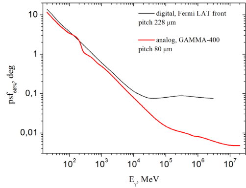
Figure 6. The dependence of the angular resolution vs the energy for: GAMMA-400 ( 80 \mu\text{m} pitch, analog readout) and Fermi-LAT ( 228 \mu\text{m} pitch, digital readout)
