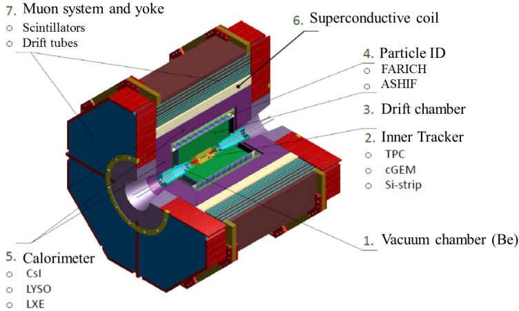
Figure 1. Conceptual design of the Super C\text{-}\tau factory detector.
