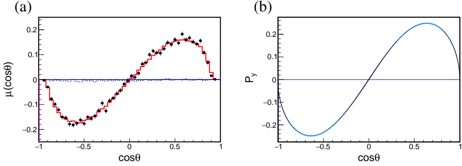
Figure 1. (a) Moment \mu(\cos \theta) as a function of \cos \theta for e^+e^- \rightarrow J/\psi \rightarrow (\Lambda \rightarrow p\pi^-)(\bar{\Lambda} \rightarrow \bar{p}\pi^+) . The points with error bars are the BESIII data, and the solid-line histogram is the global fit results. The dashed histogram shows the no polarization scenario ( \mathcal{W}(\xi; 0, 0, 0, 0) \equiv 1 ). (b) Polarization of \Lambda as a function of \cos \theta calculated using the determined values of \alpha_\psi and \Delta\Phi .
