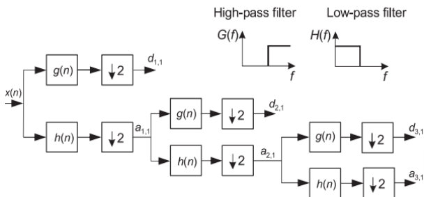
Fig. 5. An example of signal decomposition by the DWT. The operator \downarrow 2 means down-sampling by two [19].
