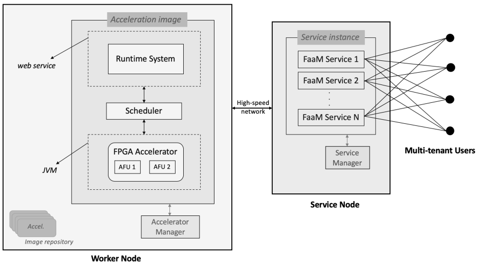
Fig. 1. High-level overview of the FaaS architecture.
