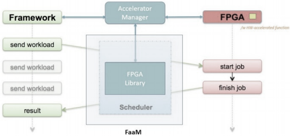
Fig. 3. Integrating frameworks with FaaSM.
