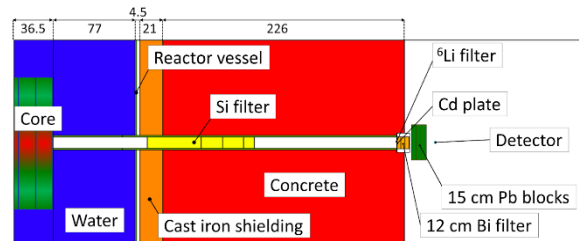
Fig. 2. The experimental arrangement in the reactor laboratory. The detectors were placed along the beam axis at 1.5 m distance from the silicon filter target [1].
